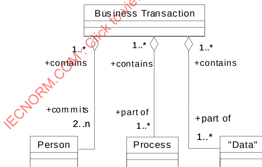
Figure F.2 — UML-based representation of “Figure F.1 - Business Transaction Model - Fundamental components”
