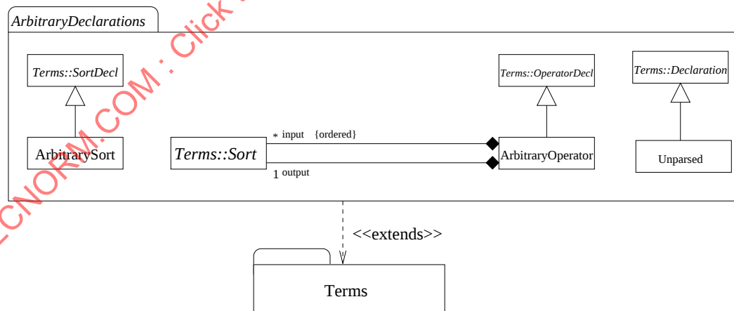
Figure 20: The package ArbitraryDeclarations
