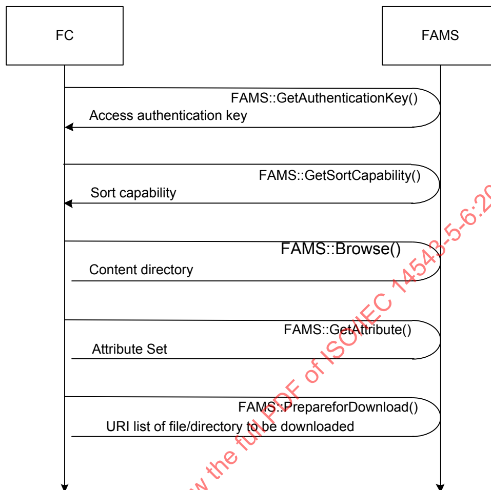
Figure 4 – File access flow
