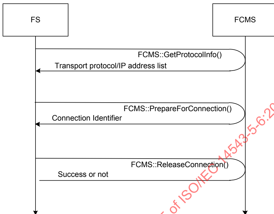
Figure 5 – Connection establishment and release flow
