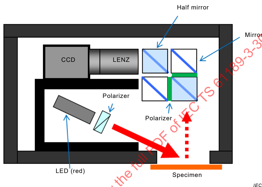
Figure A.1 – Equipment prototype
