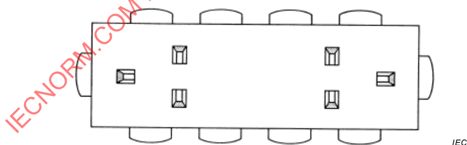
a) Microphones positioned in accordance with the 3-to-1 rule, using cardioid microphones
