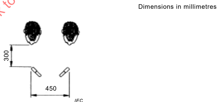
Figure 28 – A reduced 3-to-1 ratio using angled microphones
