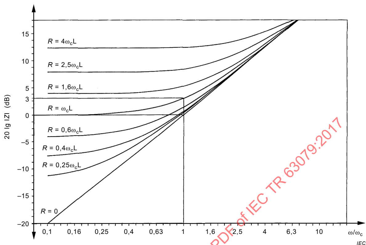
Figure 10 – Variation with frequency of the logarithm of the impedance of loops of constant inductance L , with the loop resistance R as parameter
