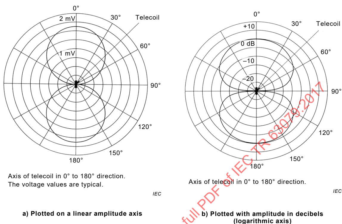
Figure 6 – Directional response of a hearing aid telecoil
