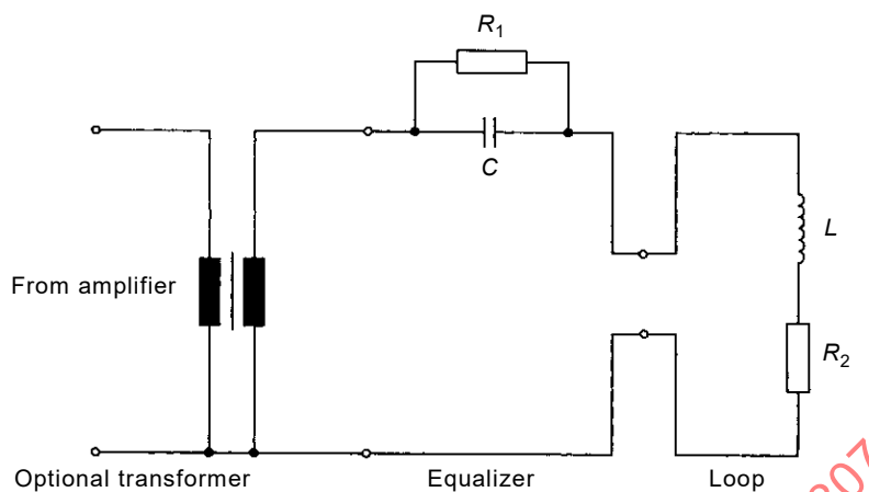
Figure C.6 – Circuit diagram of a “high-level” or Popperwell equalizer (for insertion between the amplifier and the loop)
