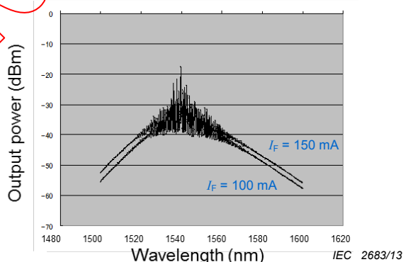
Figure 10c – SOA chip sample #3 with a gain ripple of more than 10 dB at I_F = 100 mA
