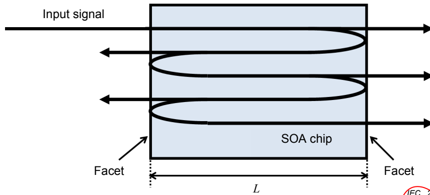
Figure 5 – Schematic diagram of the optical feedback inside the SOA chip
