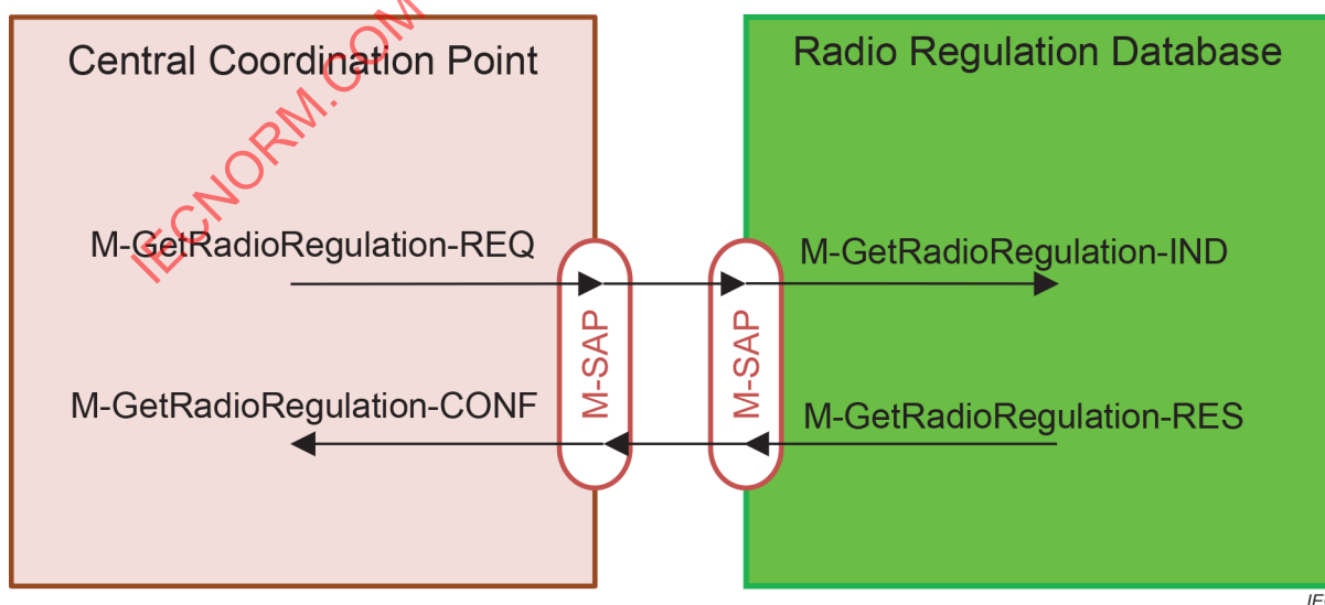
Figure 41 – Primitive flow of GetRadioRegulation service
