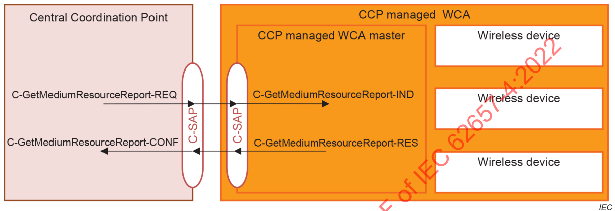
Figure 31 – Primitive flow of GetMediumResourceReport service for CMWCA
