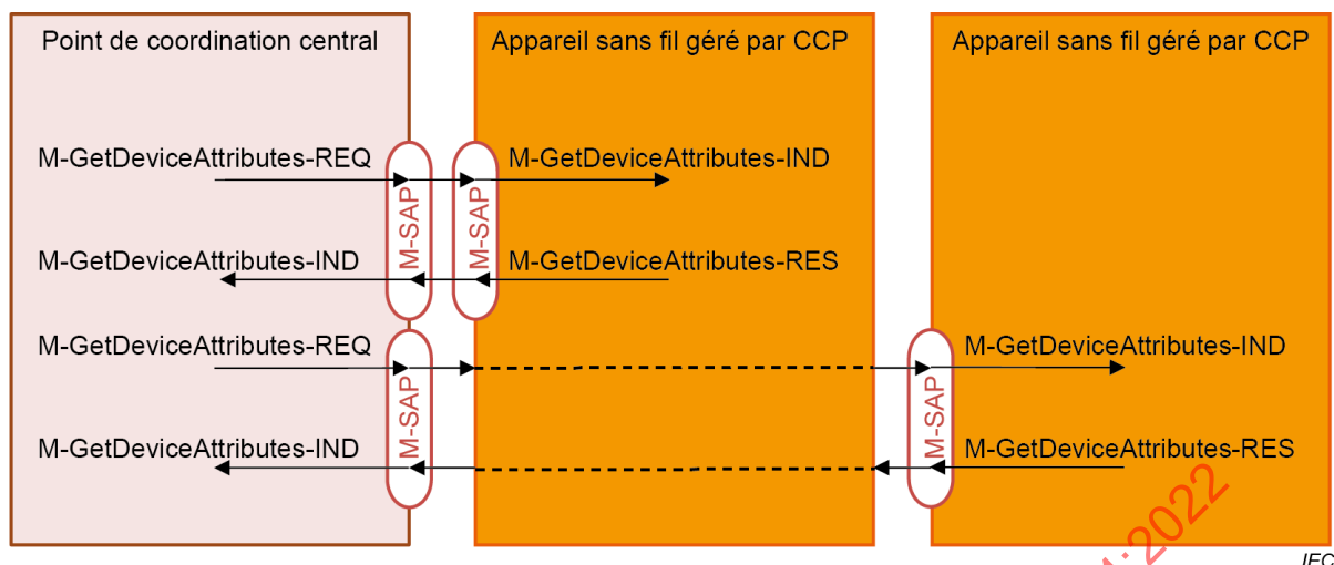
Figure 18 – Flux de primitives de GetDeviceAttributes
