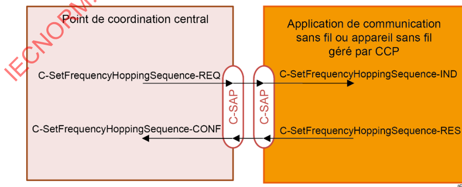
Figure 22 – Flux de primitives du service SetFrequencyHoppingSequence
