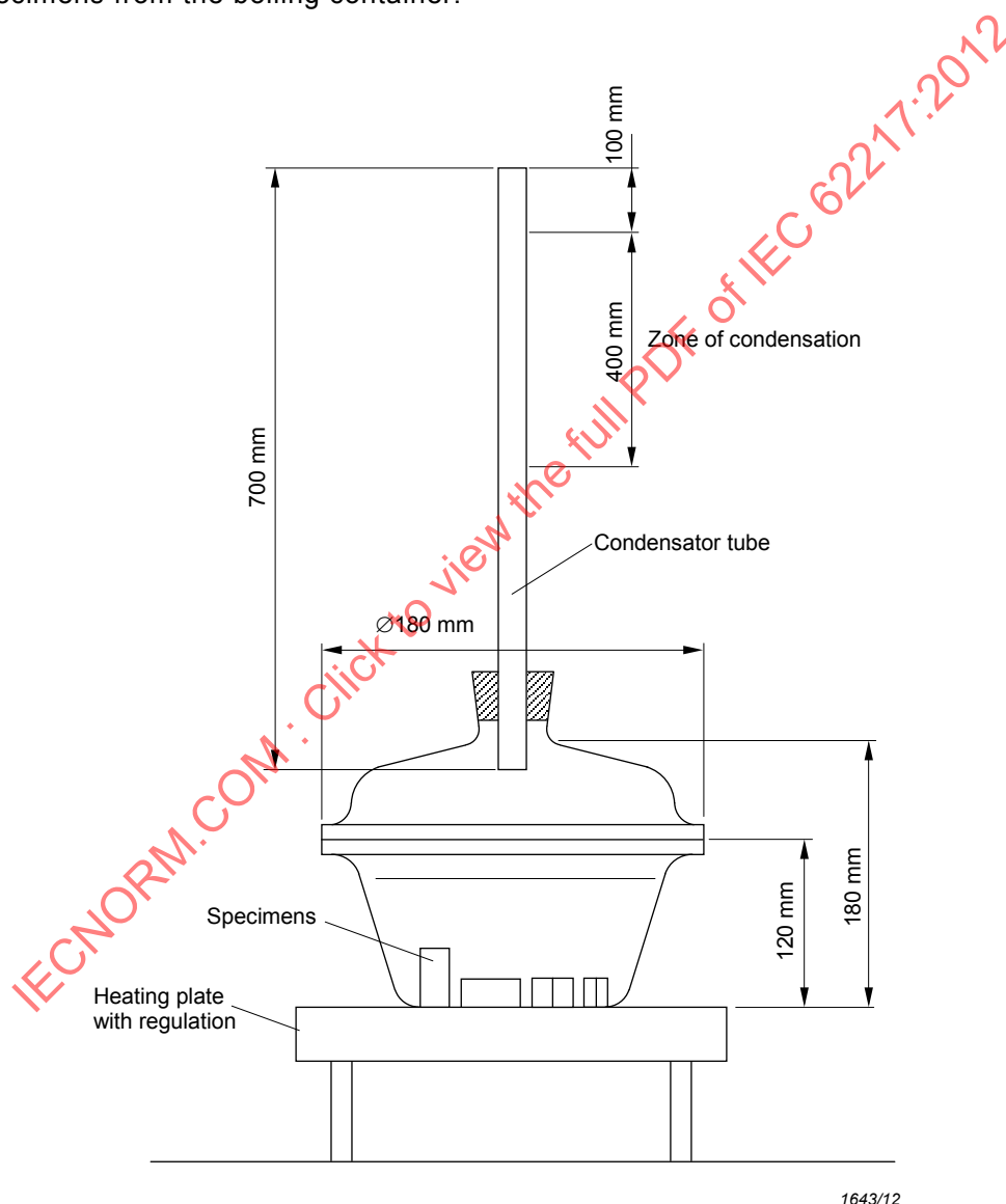
Figure 2 – Example of boiling container for the water diffusion test
