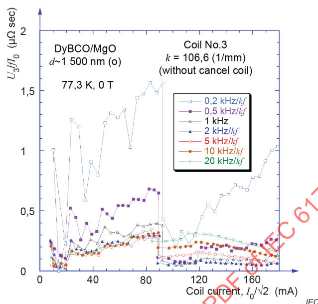
Figure B.5 – Normalized harmonic noises ( U_3/I_0 ) arising from the power source
