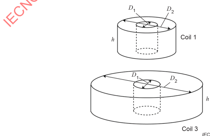
Figure 7 – Illustration of coils 1 and 3 in Table 2
