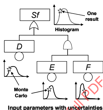
Figure B.38 – Uncertainty propagation principle
