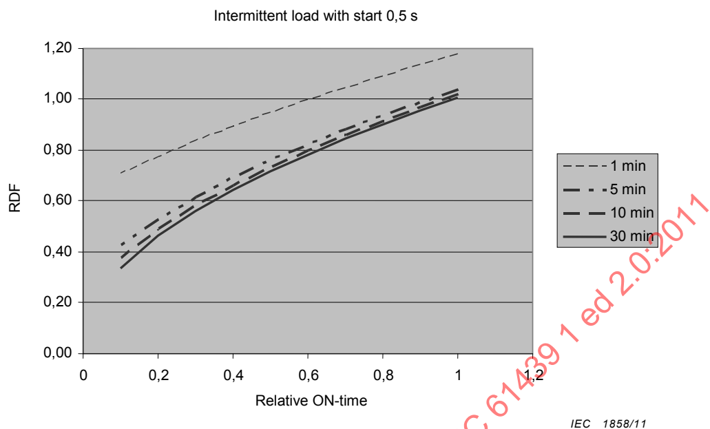
Figure E.7 – Example graph for the relation between the equivalent RDF and the parameters at intermittent duty at t_1 = 0,5 s, I_1 = 7 \cdot I_2 at different cycle times
