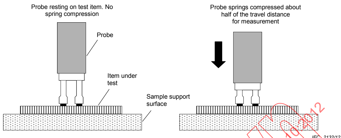
Figure 4 – Spring compression for measurement
