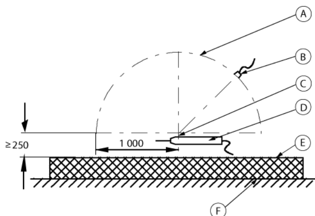
Figure 7a – Positioning of the voltage detector in the test set-up
