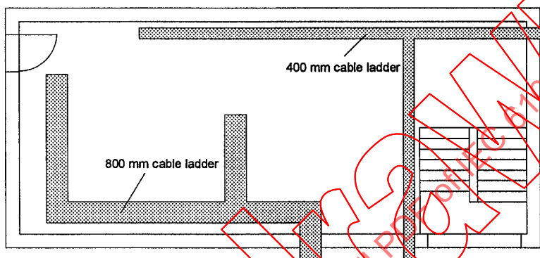
Figure 2b) – Basic drawing with cable routing added
