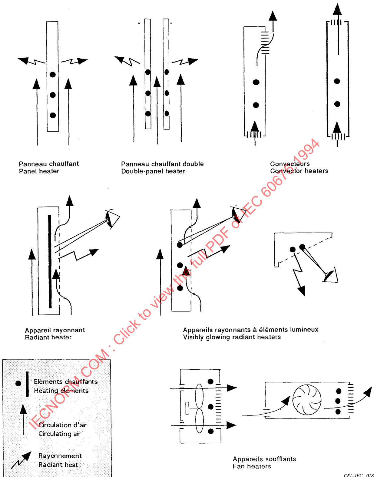
Figure 1 – Exemples de types d'appareils Examples of types of heaters
