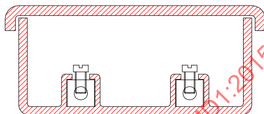
Figure AA.1a – Enclosures with integrated clamping units according to 7.101.1
