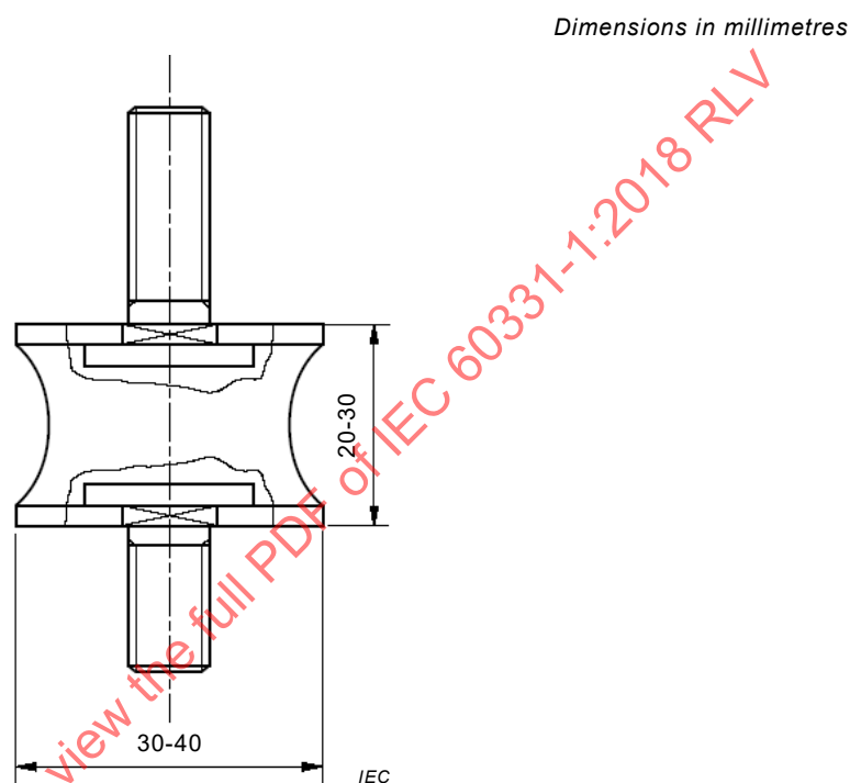
Figure 4 – Typical rubber bush for supporting the test ladder
