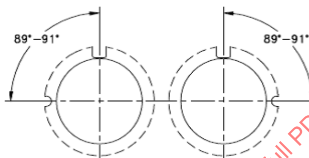
P32d-5 PK32d-5
