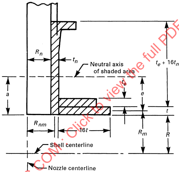
(c) Case A Nozzle With Reinforcing Pad
