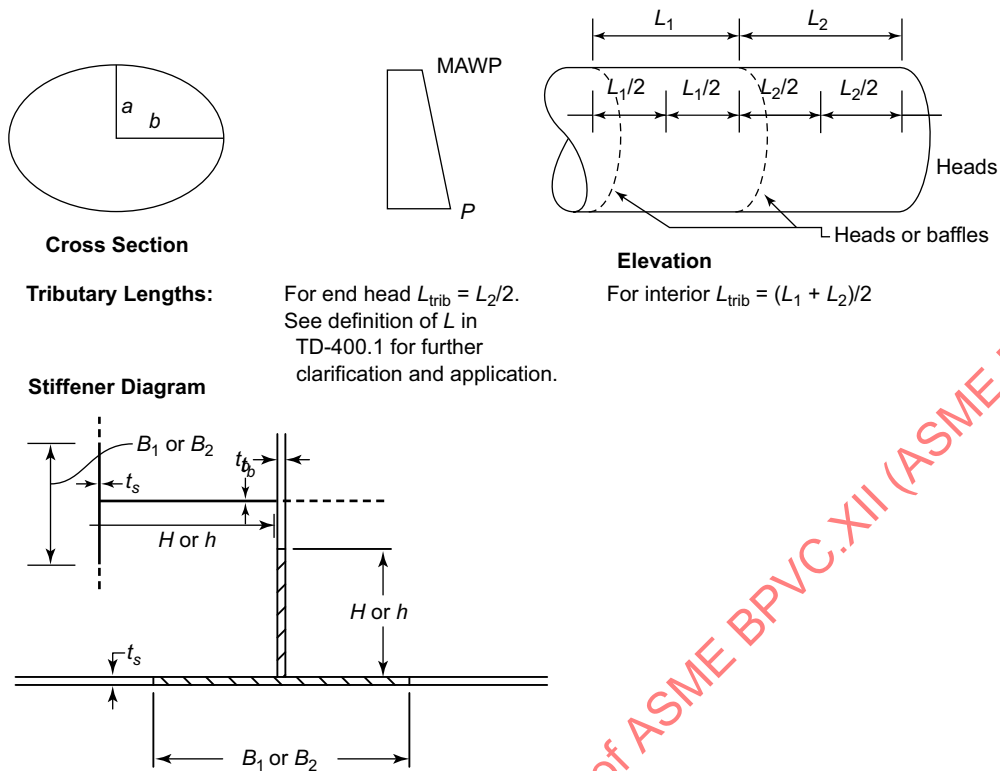
Figure VIII-2-3 Noncircular Cargo Tank Structural Properties
