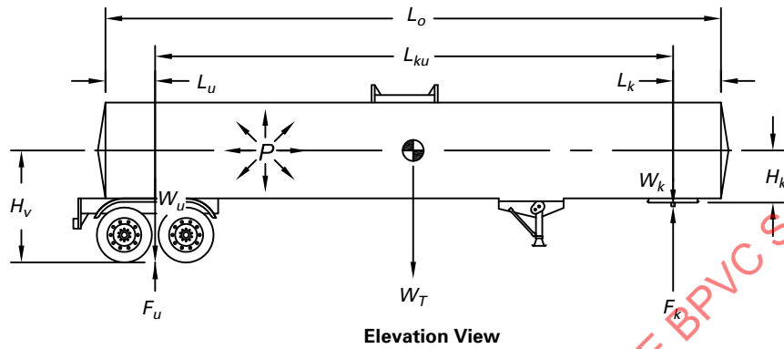
(a) Static Load Condition A
