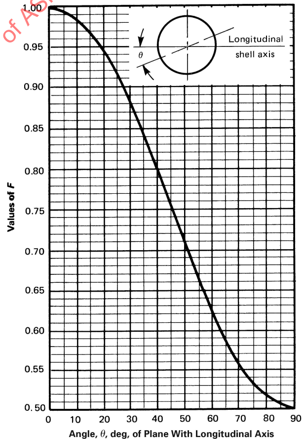
Figure TD-610.3-1 Chart for Determining Value of F , as Required in TD-610.3
