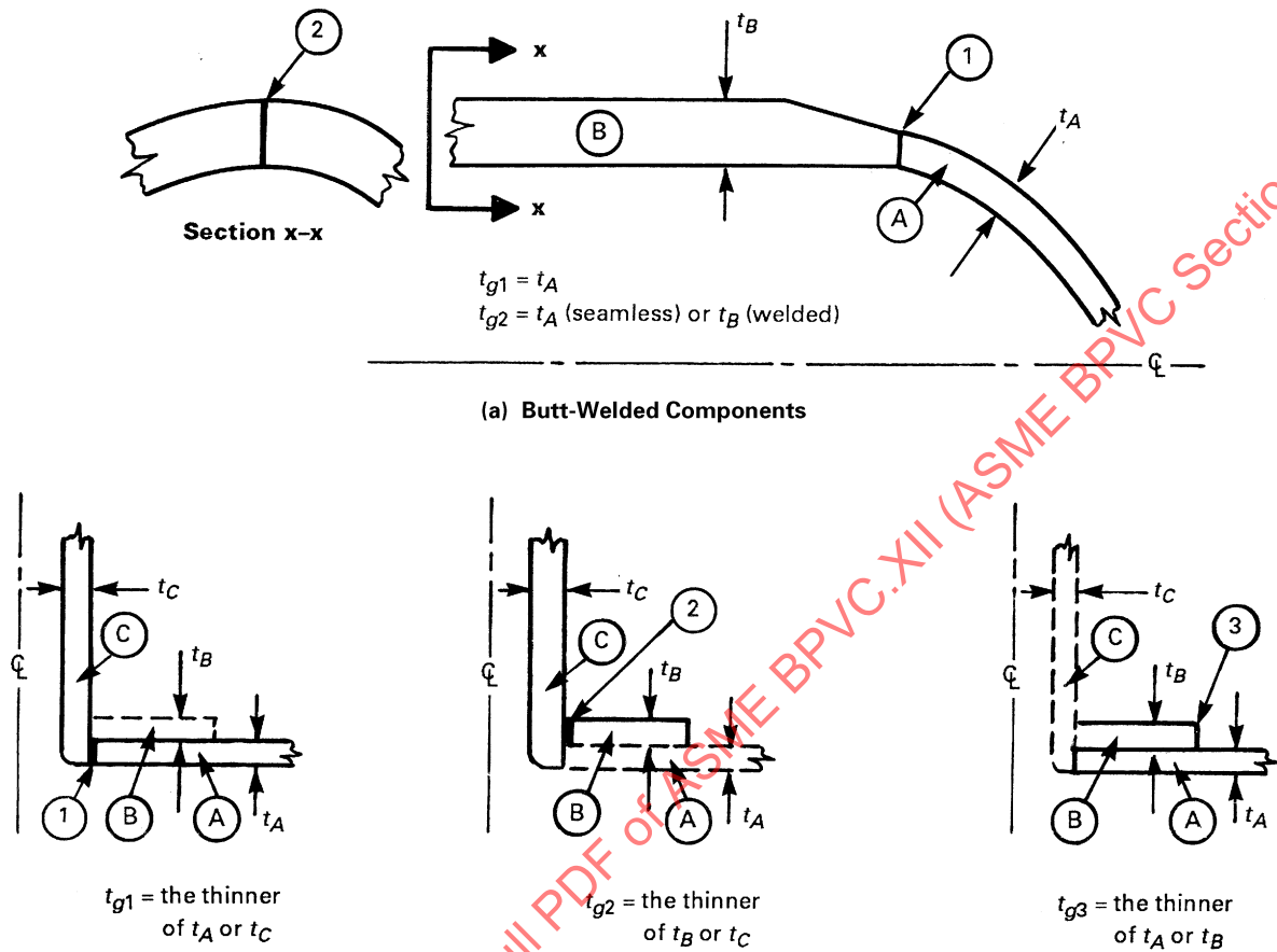
Figure TM-240.1-2 Some Typical Tank Details Showing the Governing Thicknesses as Defined in TM-240.1
