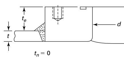
Figure TD-640 Some Representative Configurations Describing the Reinforcement Dimension, t_e , and the Opening Dimension, d
