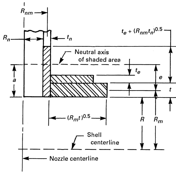
(a) Case A Nozzle With Reinforcing Pad
