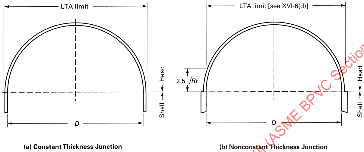
Figure XVI-6-3 Limits for Hemispherical Head
