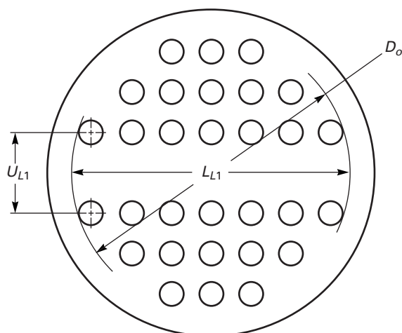
Figure UHX-11.5.1-2 Typical Untubed Lane Configurations
