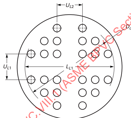
Figure UHX-11.5.1-2 Typical Untubed Lane Configurations
