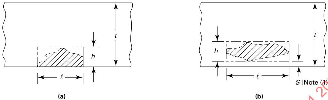
Surface Indications
