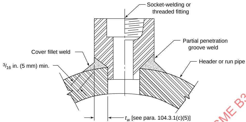
(a) Branch Connection Typical Partial Penetration Weld
