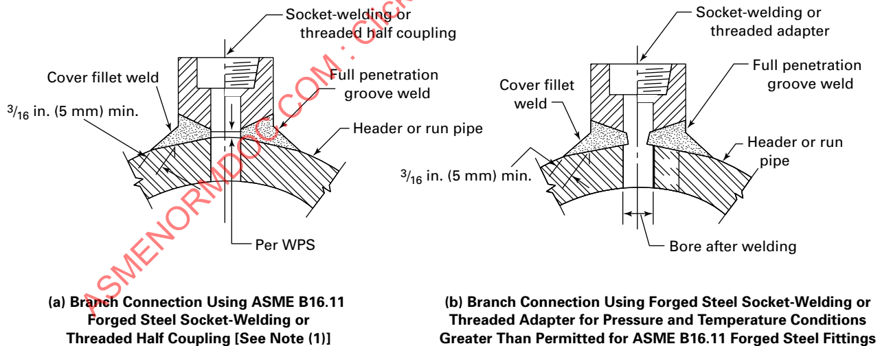
Figure 127.4.8-6 Typical Full Penetration Weld Branch Connections for NPS 3 (DN 80) and Smaller Half Couplings or Adapters
