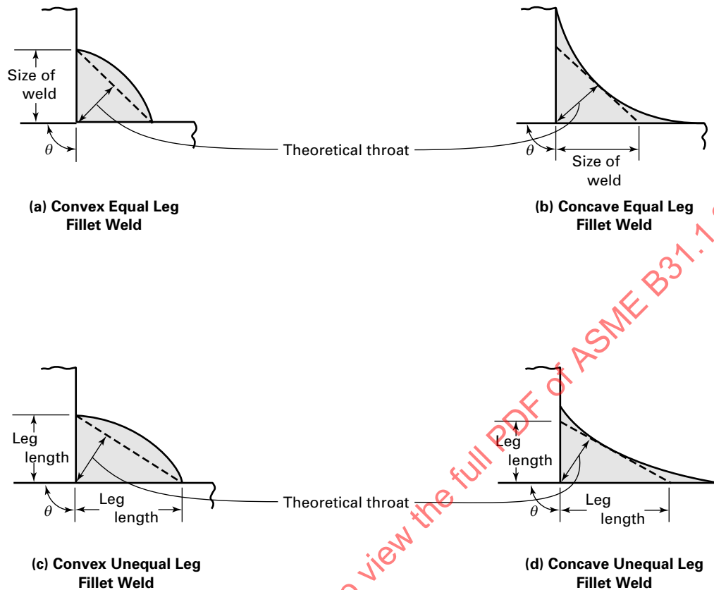
Figure 127.4.4-1 Fillet Weld Size
