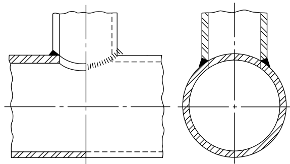
Figure 127.4.8-1 Typical Welded Branch Connection Without Additional Reinforcement
