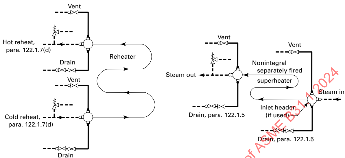
Figure 100.1.2-5 Code Jurisdictional Limits for Piping — Reheaters and Nonintegral Separately Fired Superheaters
